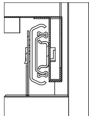
DETAIL K SCALE 1 : 2
